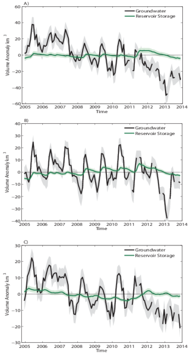
Figure 3. Monthly anomalies ( \text{km}^3 ) of groundwater storage (black) and of surface reservoir storage (green) for (A) the entire Basin (trend: -5.6 \pm 0.4 \text{ km}^3 \text{ yr}^{-1} ) and Lakes Powell and Mead combined (trend: -0.9 \pm 0.6 \text{ km}^3 \text{ yr}^{-1} ); (B) the Upper Basin (trend: -1.7 \pm 0.4 \text{ km}^3 \text{ yr}^{-1} ) and Lake
