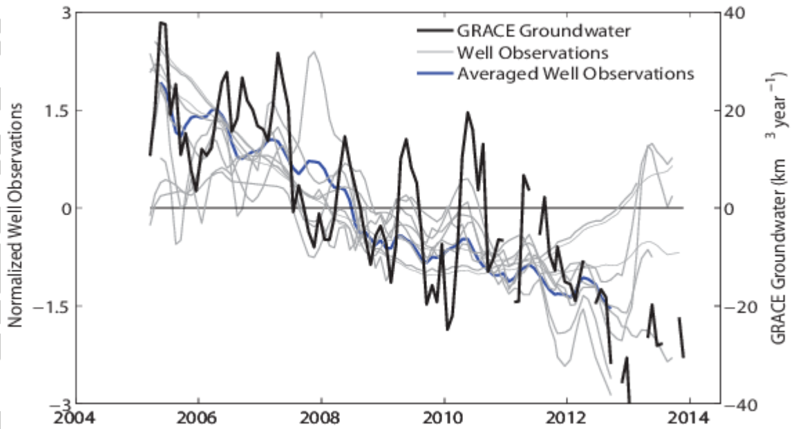
Figure 4. Entire Basin comparison between GRACE groundwater storage anomalies (black line) in \text{km}^3 and monthly USGS well observations (blue line is average of gray lines). Because specific yield information is not available for all wells, we normalize each well time series by its standard deviation and then average (in blue). Selected well observations were only available from March 2005 to October 2012; thus, we calculated the average over this time period.
