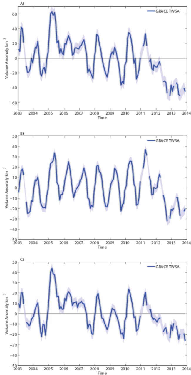
Figure 2. Monthly anomalies (deviations from the mean of the study period) of total water storage (TWSA) for (A) the entire Basin; (B) the Upper Basin; and (C) the Lower Basin, from January 2003 to November 2013 (i.e. the full GRACE RL05 record available at writing). The three TWSA estimates were calculated independently using basin specific scaling. Anomaly errors are shown in light blue shading. There are inconsecutive gaps in the GRACE data record,
